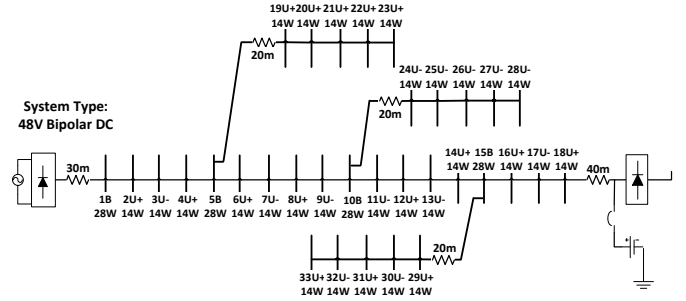
Fig. 9. System Diagram of Bipolar DC Radial 33-Bus Network
