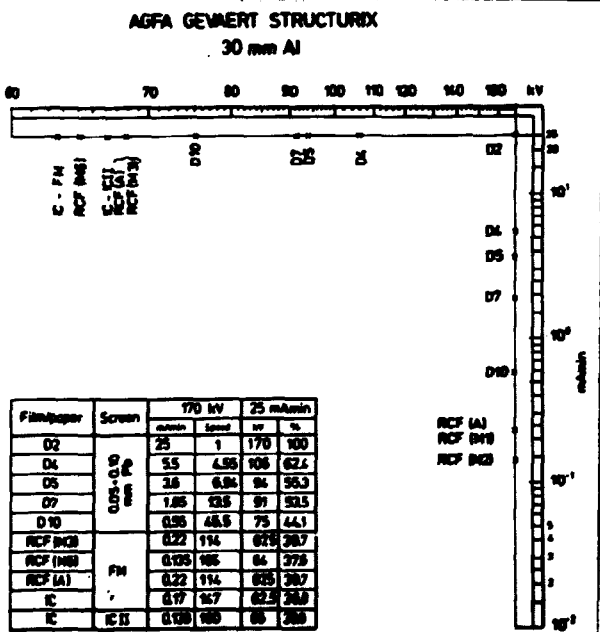
Fig. 4. Constant exposure and constant kilovoltage exposures for Kodak Industrex and Agfa-Gevaert Structurix systems
