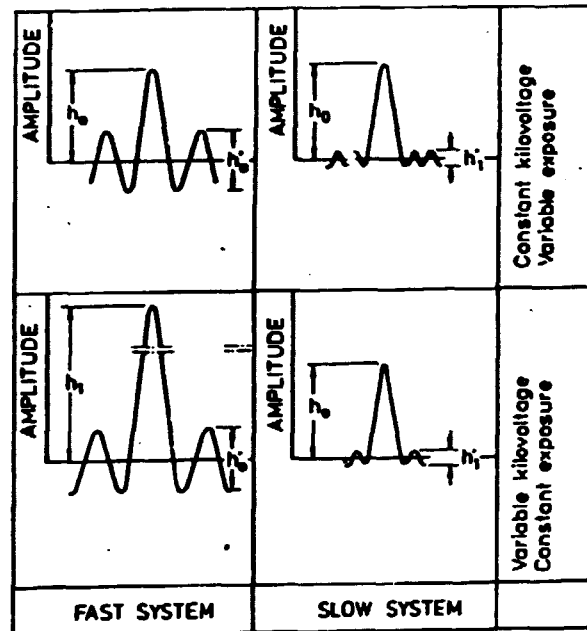
Fig. 3. Comparison between the constant kilovoltage and constant exposure technique
