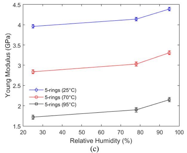
Fig. 7. Young's Modulus versus relative humidity in different temperature for (a) 2-ring, (b) 3-ring, and (c) 5-ring mPOF.
