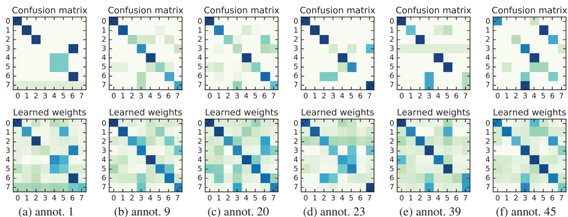
Figure 3: Comparison between the learned weight matrices \mathbf{W}^T and the corresponding true confusion matrices.
