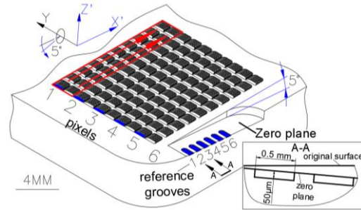
Fig. 4. The Z axial positioning accuracy test.
