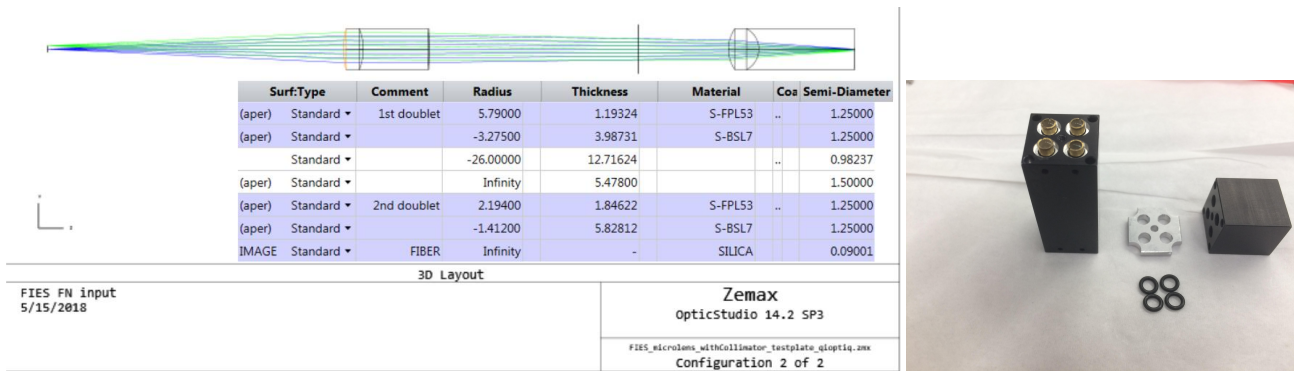
Figure 1: FIES FN-system design that convert the f/11 telescope beam to f/4.8 (left). All lenses have a diameter of 2.5 mm and are held in a thin brass tube. Due to optical constrains, all fibers had to sit closely (6 mm distance) together (right).
