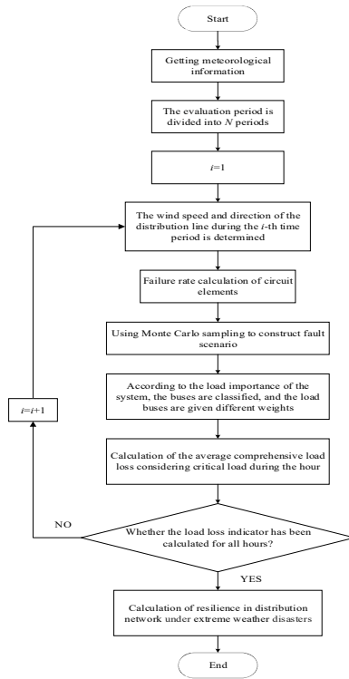
FIGURE 1. Detailed process of evaluation method
