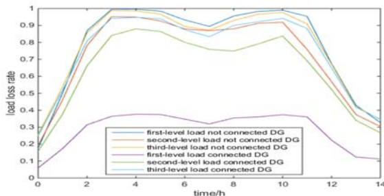
FIGURE 4. Load loss rate of system buses under the typhoon weather
