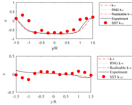
Fig. 15. Velocity profiles at the azimuth position of 30° for four turbulence models.
