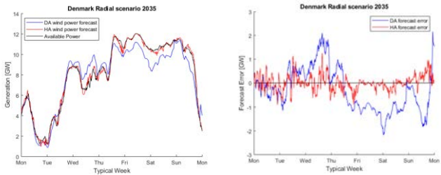
Figure 5 Forecast vs. available wind power in a typical week simulated for 2035
