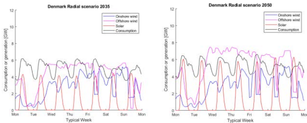
Figure 3 Generation and consumption in a typical week
