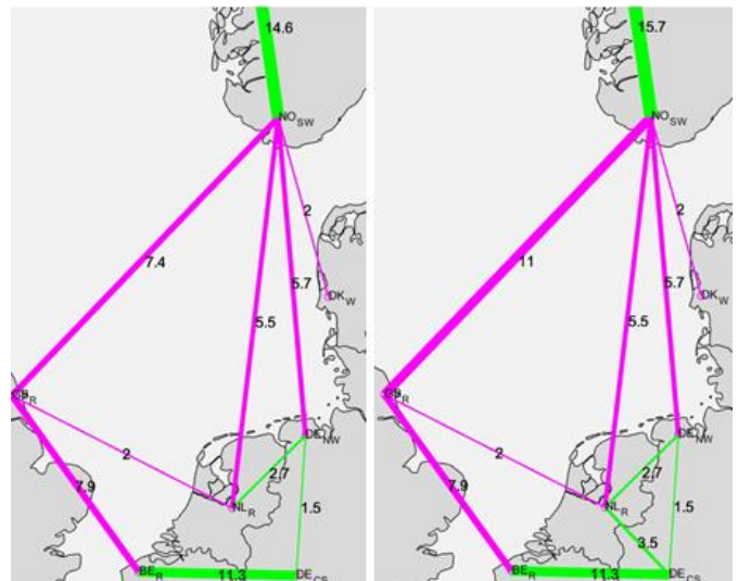
Figure 2. Endogenous transmission investments in 2035 (left) and accumulated endogenous transmission investments by 2050 (right) in GW. On-land lines are drawn in green, and HVDC offshore lines in magenta.
