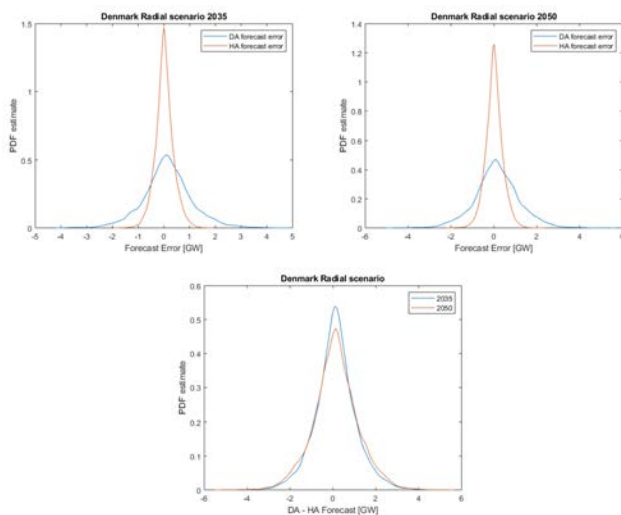
Figure 8 Probability density function for wind power forecast error
