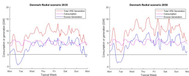
Figure 4 Total VRE generation, consumption and residual generation in a typical week simulated for 2035 and 2050
