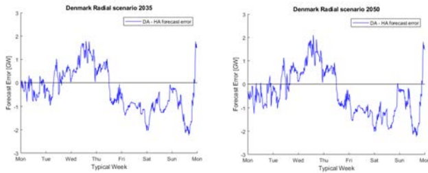
Figure 7 Difference between day-ahead and hour-ahead wind power forecast error
