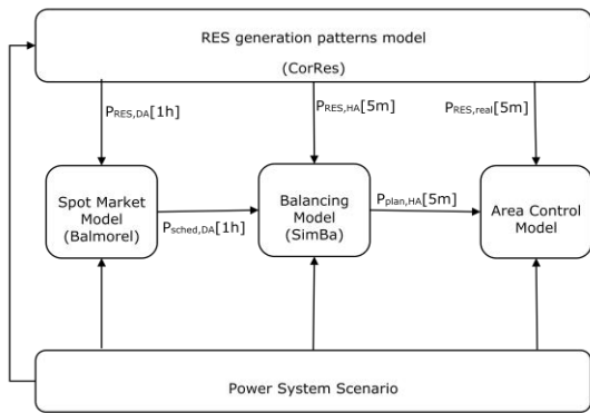
Figure 1 Balancing Model Tool Chain
