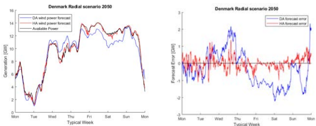
Figure 6 Forecast vs. available wind power in a typical week simulated for 2050
