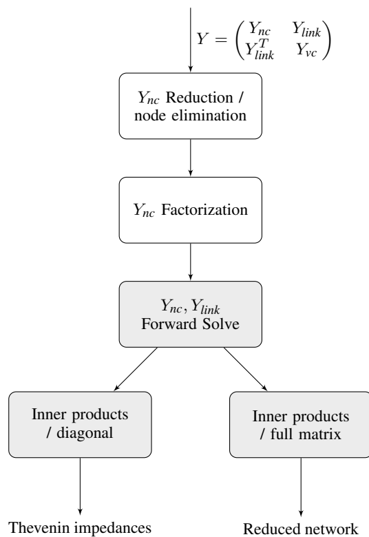
Fig. 1: The reduce-factor-solve approach, see also Algorithm 1. The full system admittance matrix Y is partitioned into the voltage controlled Y_{vc} , non-voltage controlled Y_{nc} , and link Y_{link} parts. The algorithm performs a fill-in limiting reduction/node elimination followed by a factorization of Y_{nc} . Computation of Thevenin impedances (left) or fully reduced network (right) follows after a forward solve and inner product computations. The grayed boxes represent fully parallelizable parts of the algorithm, while the white boxes are primarily serial allowing only fine-grained parallelization.
