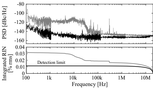
Figure 7: Amplitude noise of the SHG light from both nonlinear crystals (top). Cumulative integrated RIN starting at 10 MHz and ending at 100 Hz (bottom). The SHG power was stabilized at 2 W ( I_{RW} = 250 mA and I_{TA} = 12 A).
