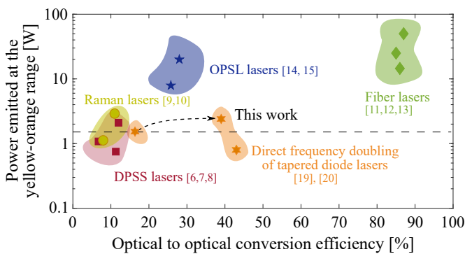
Figure 1: Attained power by different technologies at the yellow-orange range as a function of the optical to optical conversion efficiency. The colored areas were plotted to guide the eye.
