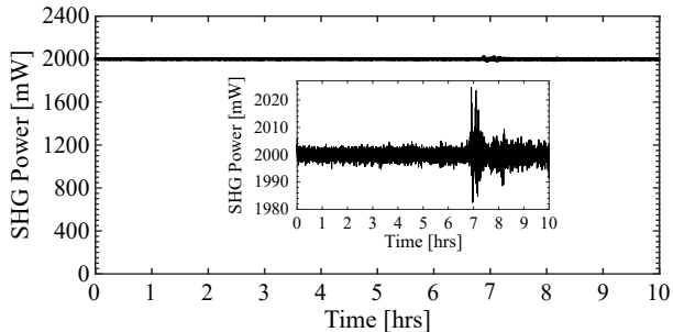
Figure 6: Power stability over 10 hours. The inset shows the same SHG power as a function of time but in a range of 45 mW. The power meter bandwidth was 100 kHz.
