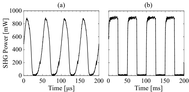
Figure 9: Modulation results for two pulse durations T_{pulse} = 25 \mu\text{s} (a) and T_{pulse} = 25 \text{ms} (b). The CW conditions were I_{RW} = 300 mA, I_{TA} = [2, 10] A. The temperature of the PPLN crystal was T_{C1} = 34.8^\circ\text{C} .
