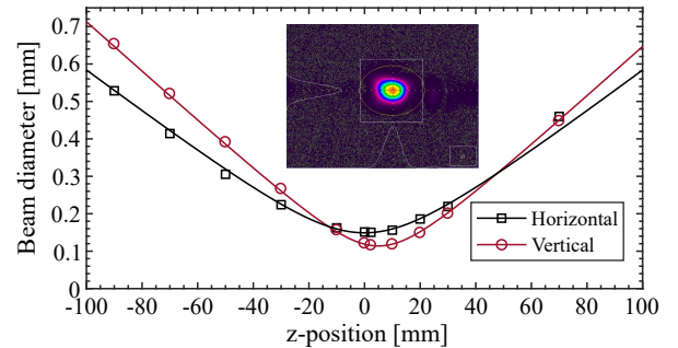
Figure 5: Beam diameters according to the second order moments at 2.7 W yellow light. The inset shows an image of the beam at the focus.
