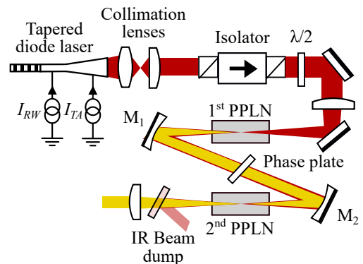
Figure 2: Schematic representation of the experimental setup for generating yellow light.
