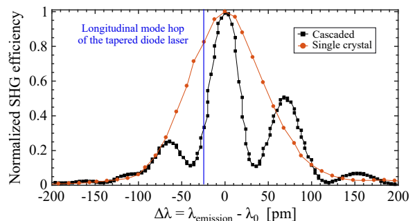
Figure 8: Normalized SHG efficiency for the single crystals (orange circles) and for the cascaded configuration (black squares) relative to the wavelength drift \Delta\lambda . \Delta\lambda is defined as the diode emission wavelength \lambda_{emission} minus the central wavelength \lambda_0 = 1153 nm. Solid lines are drawn to guide the eye.
