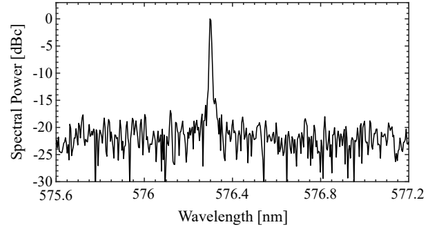
Figure 4: Optical spectrum at the maximum SHG power. The driving currents for the tapered diode laser was I_{RW} = 250 mA and I_{TA} = 12 A. The temperature of the crystals were T_{C1} = 36^\circ\text{C} and T_{C2} = 35.7^\circ\text{C} .
