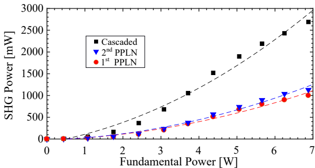
Figure 3: SHG power as a function of the fundamental IR power. The temperature of the crystals was adjusted for each point of the curve.
