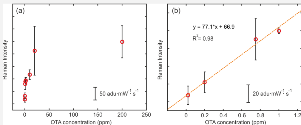
Figure 2. A) Plot of Raman intensity as a function of OTA concentration. The error bar represents the standard deviation of triplicate measurement; B) Calibration curve of OTA in concentration range between 0.02 to 1 ppm; error bar represents the standard deviations of three independent measurements.
