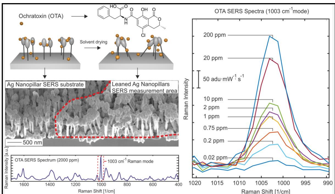
Figure 1. Left: schematic illustration of direct ochratoxin A (OTA) detection using leaning silver-capped silicon nanopillar SERS substrates. A droplet of analyte is deposited on the SERS substrate and left for drying. As a solvent evaporates, capillary forces pull the Ag nanopillars together forming microsized clusters that trap OTA in the vicinity of the so-called electromagnetic “hot spots” [5]. Right: OTA SERS spectra for concentrations varying between 0.02 – 200 ppm (1003 \text{cm}^{-1} mode).
