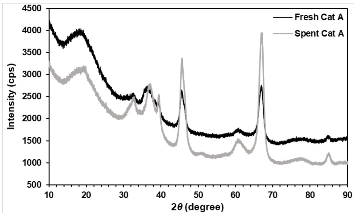
Fig. 9. XRD patterns of the fresh and spent Cu-Mn/ \delta -Al 2 O 3 catalyst.
