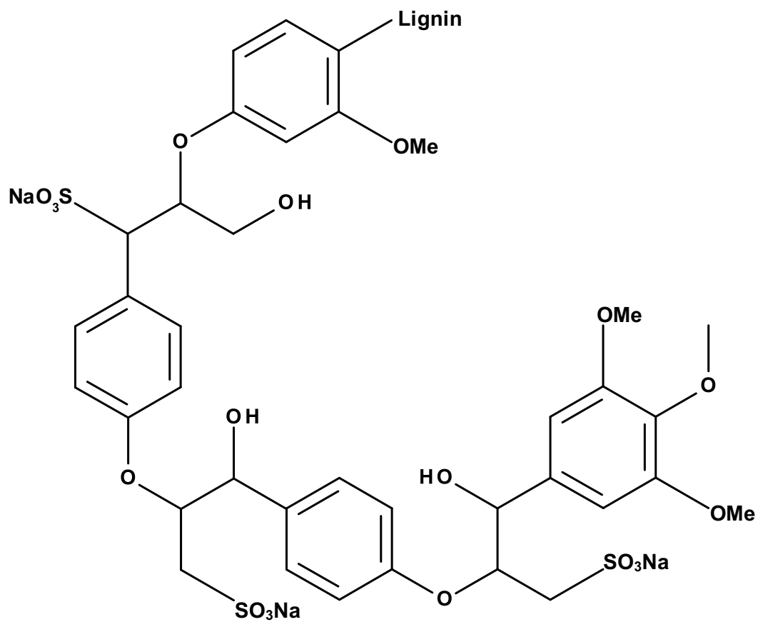
Fig. 1. Representative chemical structure of sodium lignosulphonate lignin.
