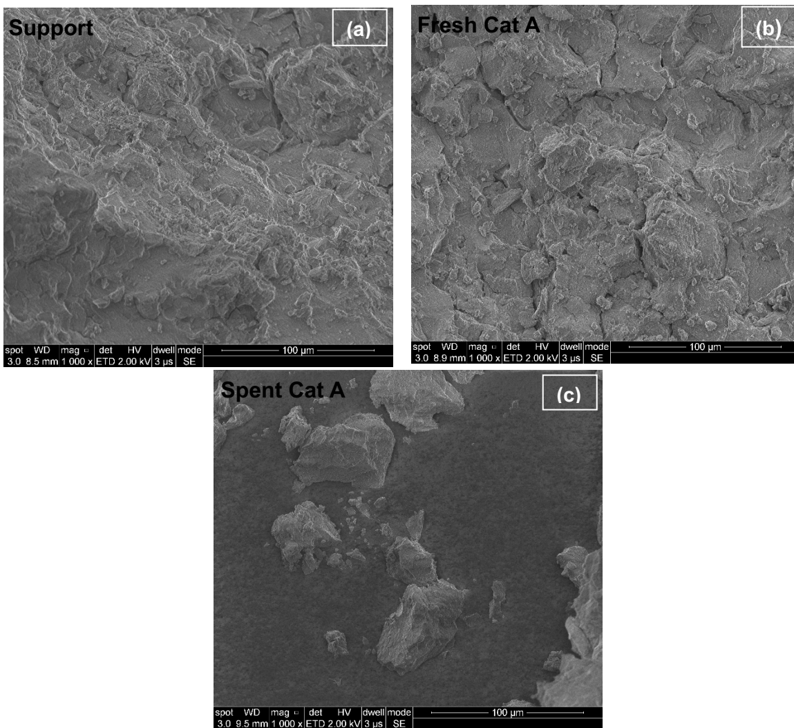
Fig. 6. SEM images of the (a) \delta -Al 2 O 3 support, (b) fresh Cu-Mn/ \delta -Al 2 O 3 catalyst and (c) spent Cu-Mn/ \delta -Al 2 O 3 catalyst.
