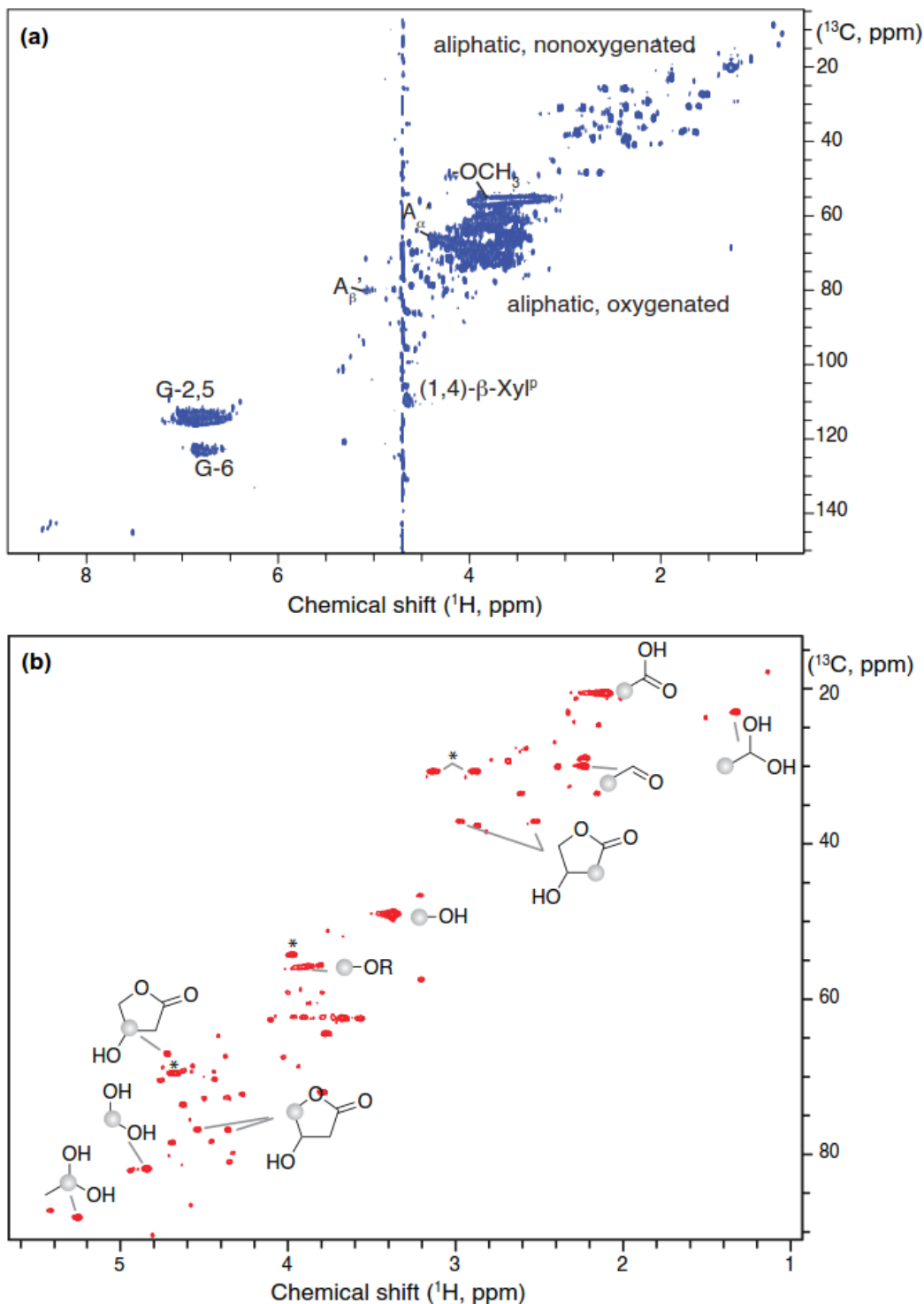
Fig. 4. Two-dimensional ^1\text{H} - ^{13}\text{C} HSQC NMR spectrum of lignosulphonate lignin substrate (a) and spectrum of identified reaction products in oxidatively depolymerised sample using \text{Cu-Mn}/\delta\text{-Al}_2\text{O}_3 catalyst, with the sphere indicating the CH group corresponding to indicated spectral signals (b). Products include methanol, formaldehyde, formic acid, acetaldehyde, acetic acid and \beta -hydroxy- \gamma -butyrolactone. The asterisk indicates a major mixture component that is tentatively assigned to the \beta -sulphonate derivative of \gamma -butyrolactone.
