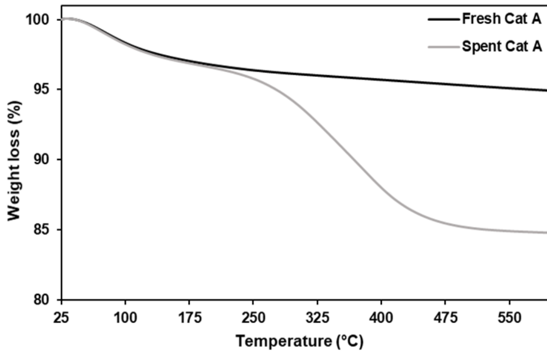
Fig. 7. TGA curves of the fresh and spent Cu-Mn/δ-Al 2 O 3 catalyst.
