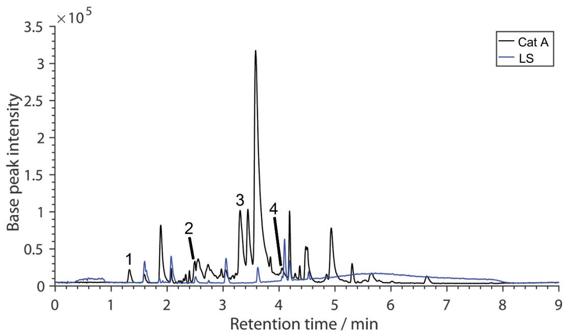
Fig. 5. Base peak ion chromatograms obtained from the SFC-MS analysis for lignosulphonate lignin (LS) substrate and oxidatively depolymerised product using Cu-Mn/ \delta -Al 2 O 3 catalyst (Cat A). Peak identities: vanillin (1), p -hydroxybenzaldehyde (2), vanillic acid (3) and p -hydroxybenzoic acid (4).
