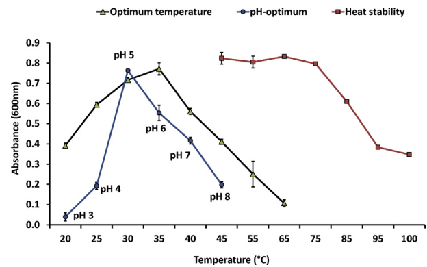
Fig. 2 – Characterization of optimum temperature and pH indicate a typical fungal enzyme profile. However, temperature stability was exceptionally high: Stable up to 70C; 40% residual activity of intact protein, active at 100C.
