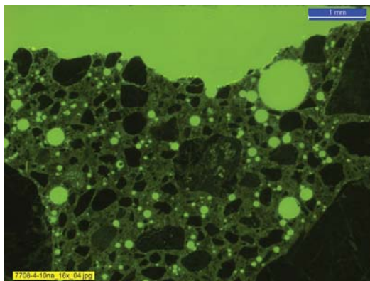
516 Figure 7: Concrete surfaces after exposure to freezing and thawing.
