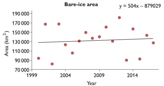
Fig. 4. End-of-melt-season bare-ice area for the Greenland ice sheet for the years 2000–2017.
