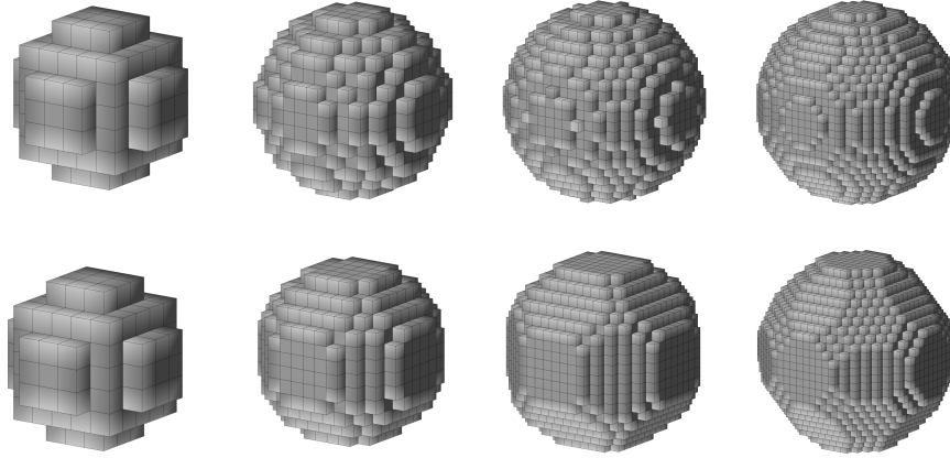
Fig. 4: Discretized spheres (top) and their zonohedral approximations (bottom). The radii are (left to right): 3, 6, 9, and 12 voxels.
