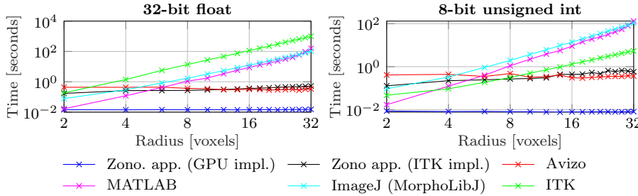
Fig. 10: Comparison of run times for different implementations of dilation with a spherical structuring element shown in a log-log plot. Benchmarks were run on a volume of size 100 \times 100 \times 100 .
