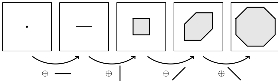
Fig. 1: Successive dilations with line segments. The resulting shape approximates a disk.
