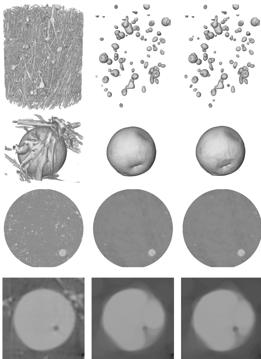
(a) Original data. (b) Opening with discretized sphere. (c) Opening with zonohedral approximation.
