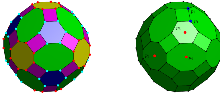
(a) Faces/vertices with the same color are equivalent with respect to the distance from the origin. (b) Points needed for the directed Hausdorff distance. Blue are vertices, red are face centers.
