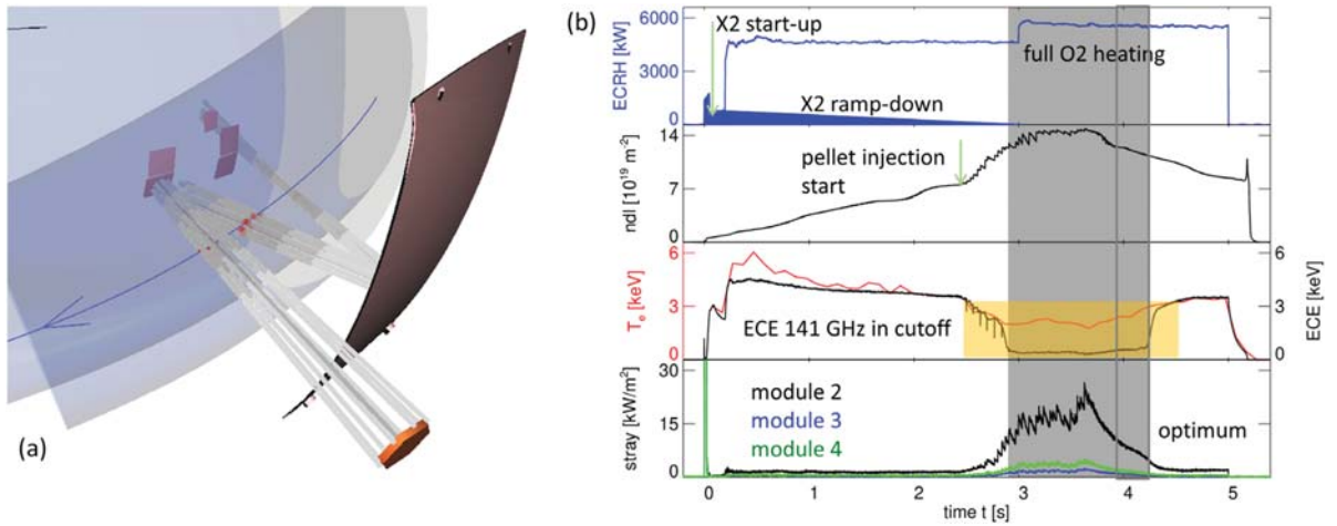
Figure 3. (a) Multi-pass absorption scheme using tungsten reflector tiles with holographic grating, mounted on the inner and the outer sides of the in-vessel system. (b) O 2 -mode heating scenario showing from top to bottom the heating power in X- and O-mode polarization (blue), the line-integrated density, the electron density measured by Thomson scattering (red) and electron cyclotron emission (black), and stray radiation measured in the device module where the wave launcher is located (black) and in the two neighboring modules (green and blue).
