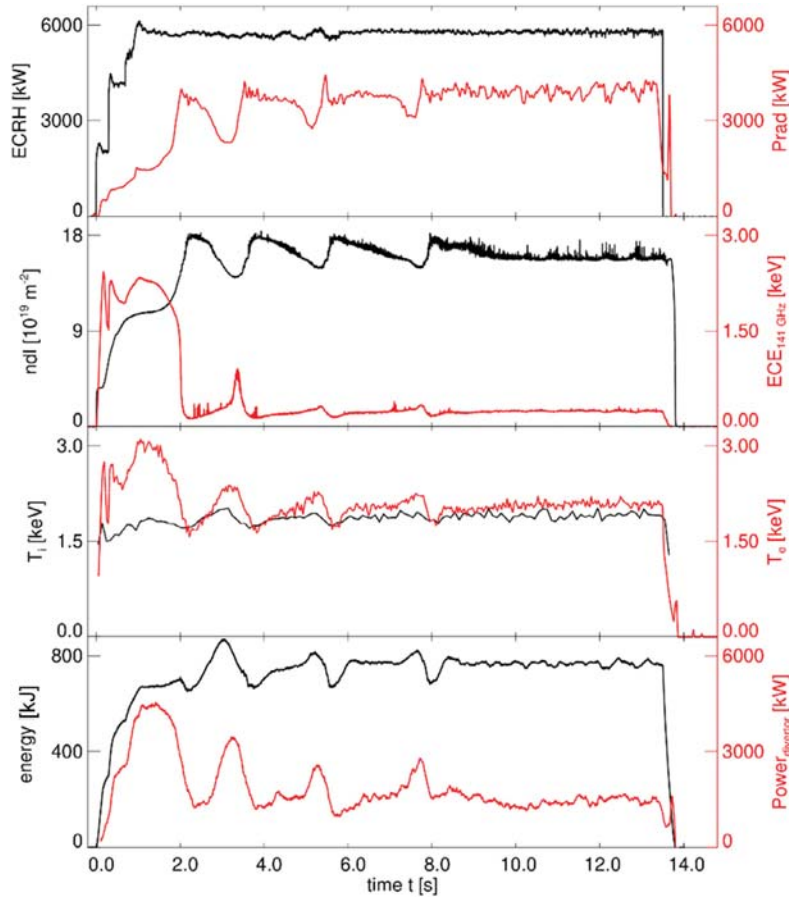
Figure 4. O 2 -mode heated long pulse high density plasma discharge. Shown are (from top to bottom, left and right scale) heating power, total radiative power, line-integrated density, electron cyclotron emission at 141 GHz, ion and electron temperature, diamagnetic energy and total divertor power load. The slow oscillations are generated by the feedback-controller. The 141GHz ECE channel runs into the cut-off after 2 s verifying the pure 140 GHz O 2 -heating.
