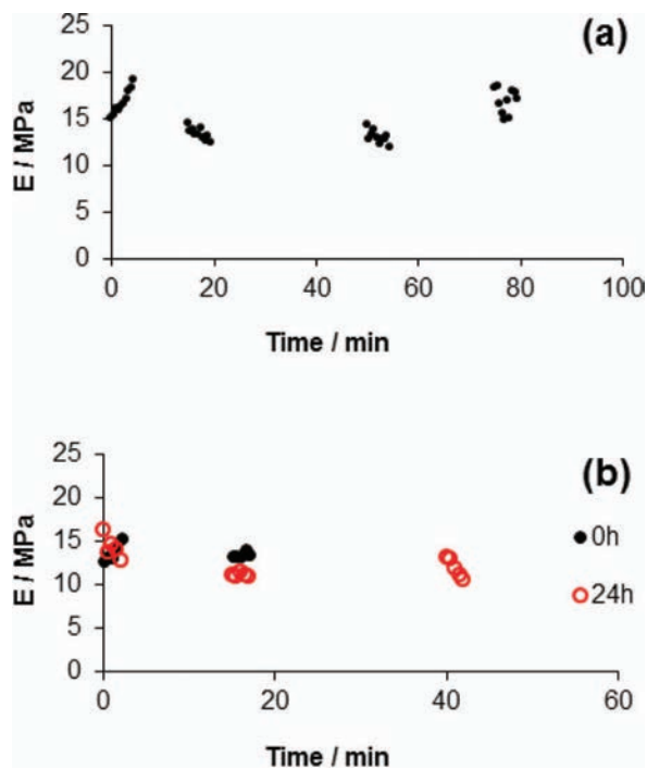
Figure 8 (A) Values of E_s at the same location on a fiber as a function of time, obtained under ambient conditions. (B) Values of E_s at the same location on a fiber as a function of time, obtained under ambient conditions at 0 h (black dots) and after 24 h of storage in a desiccator (red circles) [15].
