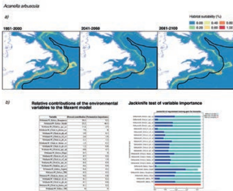
FIGURE A10.3.7 (a) Predicted probability of the suitable habitat, and (b) relative contribution of the environmental variables to the Maxent model for Acanella arbuscula in the northwest Atlantic area for the current and future climate scenarios
