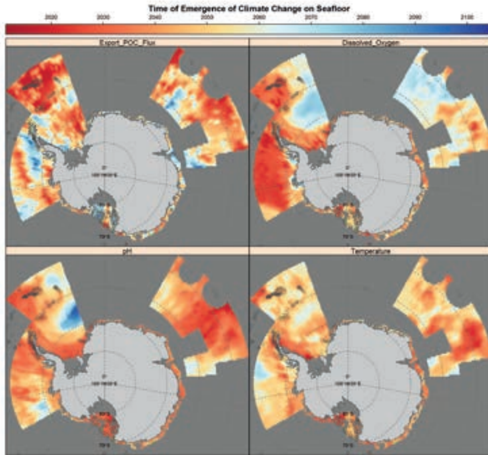
FIGURE A8.3.1 Time of emergence in CCAML
