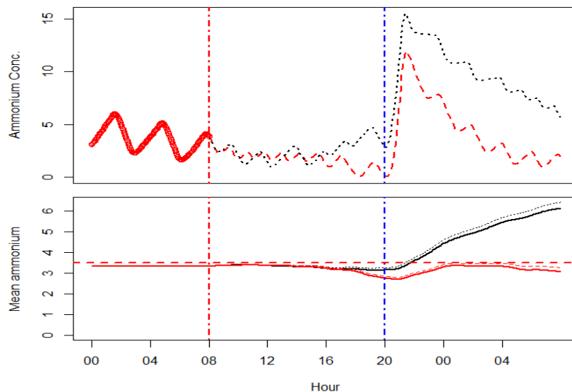
Figure 2: Control of effluent ammonium concentrations from a WWTP based on forecasts started at 08:00 (vertical red dotted line). A large incoming ammonium load is predicted at 20:00-21:00 (vertical blue dotted line), corresponding to a first-flush situation with 10 times more incoming ammonium compared to DW. The upper plot shows predicted effluent concentrations. The lower plot shows the 24-hour predicted mean of the concentrations (which are subject to regulatory constraints) with uncertainty. The dashed line is the effluent requirement of 3.5 mgN/l. Note that the black line (without weather forecast) performs worse in terms of treatment compared to the red line (with weather forecast).
