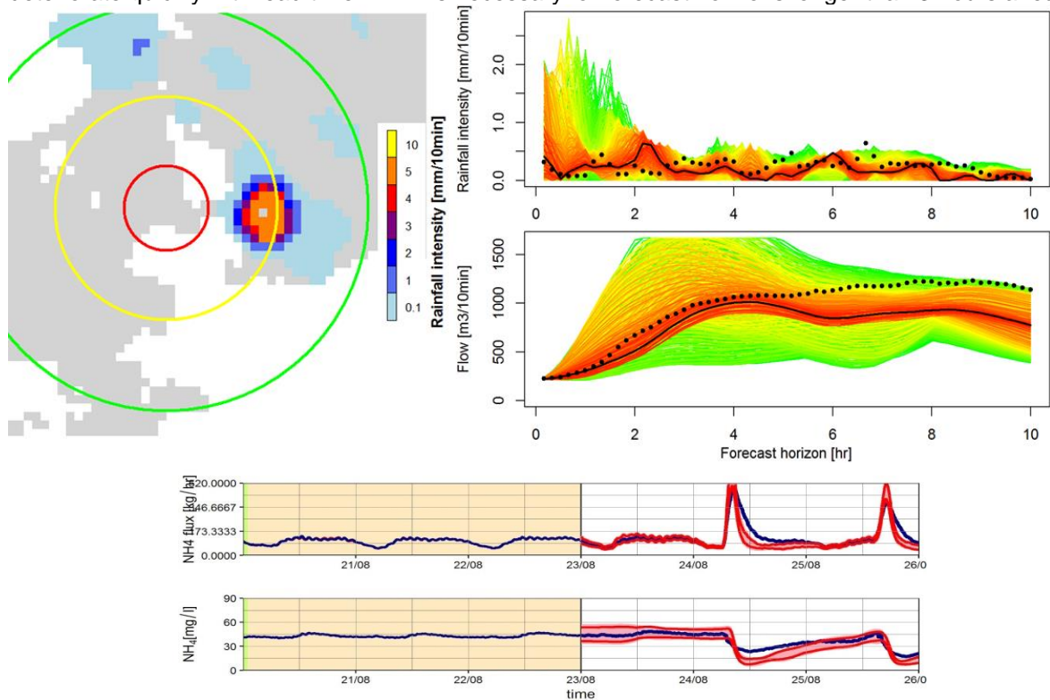
Figure 1: A single time step of a NWP-based rainfall forecast over Zealand and Southern Sweden (top, left). A time series of predicted average rainfall intensity over a sewer catchment in Copenhagen including spatial uncertainty colored by distance from the catchment (top-right-upper). A resulting ensemble flow forecast at the outlet of the sewer catchment (top-right-lower). Observed variables are indicated with black dots, while the colored lines are ensemble scenarios with red colors being rainfall (and resulting flow) predicted near the sewer catchment, while yellow and green colors are scenarios predicted to happen further away. Example of \text{NH}_4 concentration and load predictions (90% prediction bounds) based on a calibrated DW model (yellow background). Blue: measured; red: modelled (Bottom).
