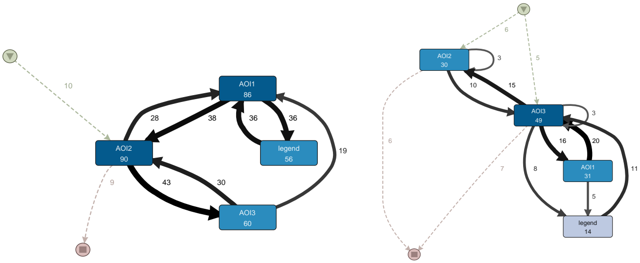
(a) Reading pattern of MPD answering Q2.
