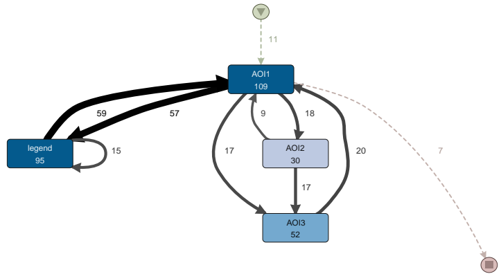
(b) Reading pattern of Rhythm-Eye answering Q2.
