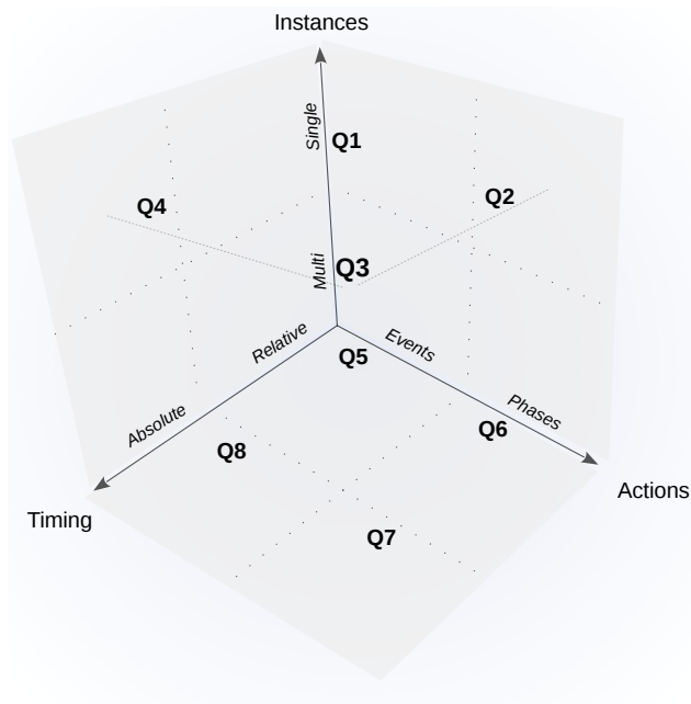
Fig. 3: Multi-Dimensional Categorization Framework for Analysis Questions regarding Process Modeling Behavior Analysis
