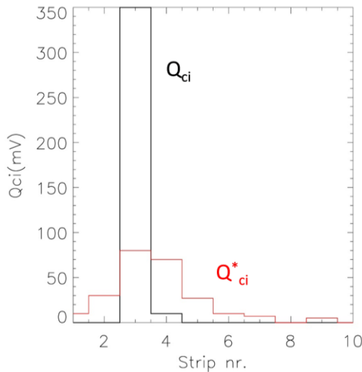
Fig. 11. The cathode strip charge distribution for an event close to cathode strip #3. Q_{ci} (black) denotes the fully integrated charge distribution whereas Q_{ci}^* (red) denotes the distribution calculated from (4).
