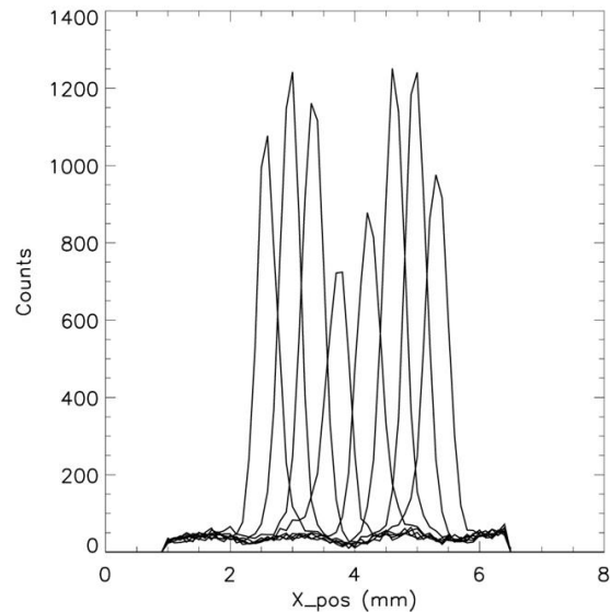
Fig. 6. X-position scans. The detector was moved in steps of 400 \mu m in front of the 200 \mu m opening of the W collimator slit.
