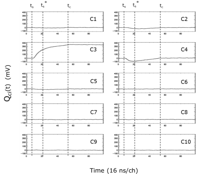
Fig. 10. The time dependence of the 10 cathode strip signals for a photon interaction event close to cathode strip #3.
