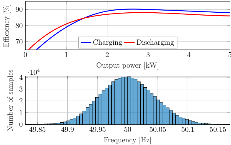
Figure 2: Upper subplot: converter efficiency curves taken from [19]. Lower subplot: histogram of frequency values in the Regional Group Nordic area.
