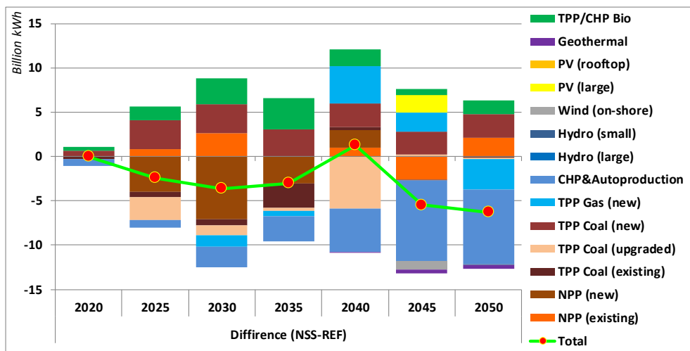
Figure 29. Differences in Electricity Generation between "National Strategies" and Reference scenarios
