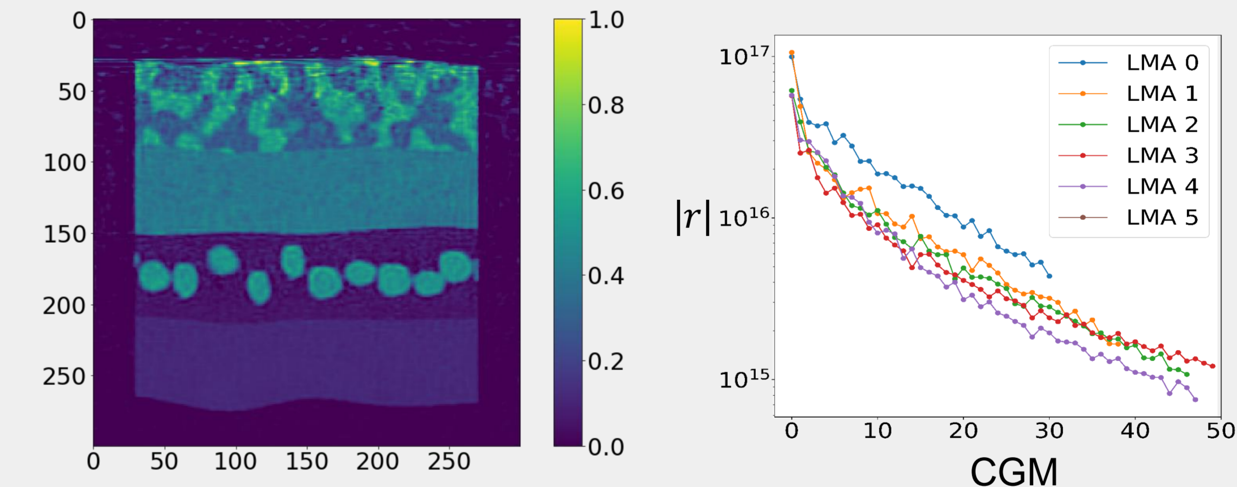
Figure 4: On the left, multi-scale reconstruction using a low-resolution image as an input; on the right: residual value over LMA and CGM iterations.
