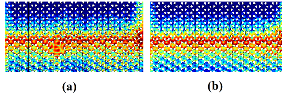
Figure 6: Acoustic pressure [30 dB SPL scale] (jet colormap) for field propagation from right to left at \nu = 20kHz along the TI-interface with (a) and without (b) a cavity.
