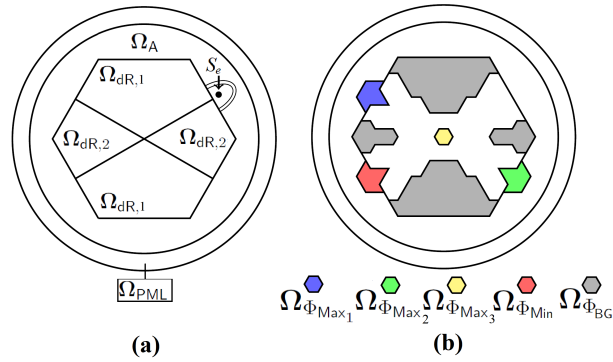
Figure 2: (a) The model domain \Omega_A \in \mathbb{R}^2 truncated using PML inside \Omega_{PML} , with two subdomains, \Omega_{dR,1} and \Omega_{dR,2} each containing a different crystal phase. S_c denotes a point source. (b) Sketch of the model domain with colors outlining different spatial regions used when formulating the design problem.
