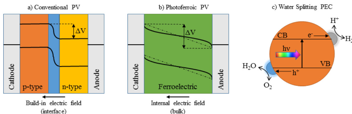
Figure 1. Illustration of conventional PV cell based on a p-n junction (a), where the splitting of the e-h pair is due to the electric field built at the interface ( \Delta V indicates the potential difference), and on photoferroic devices, for which the splitting of the photogenerated charges is enhanced by the internal polarization (b). The scheme of a photoelectrochemical cell is also shown (c).
