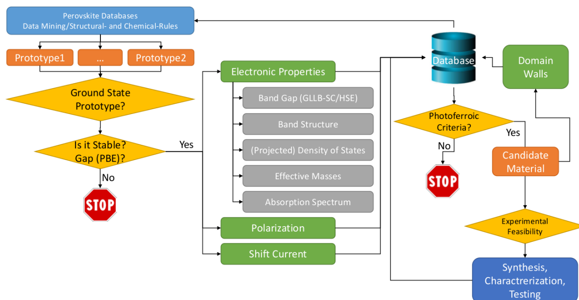
Figure 3. Example of a workflow for the computational discovery of novel photoferroic materials.
