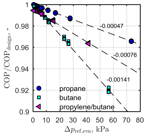
Figure 2: Normalized COP as a function of total refrigerant pressure drop in the evaporator
