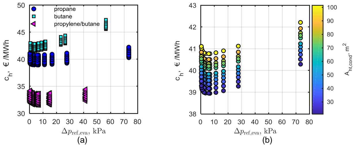
Figure 4: Specific cost of heat as function as a function of total refrigerant pressure drops in the evaporator for: (a) all fluids, (b) propane (close-up)
