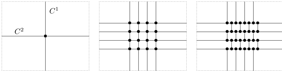
FIG. 5.1. H_1 , H_4 and H'_t on the torus
