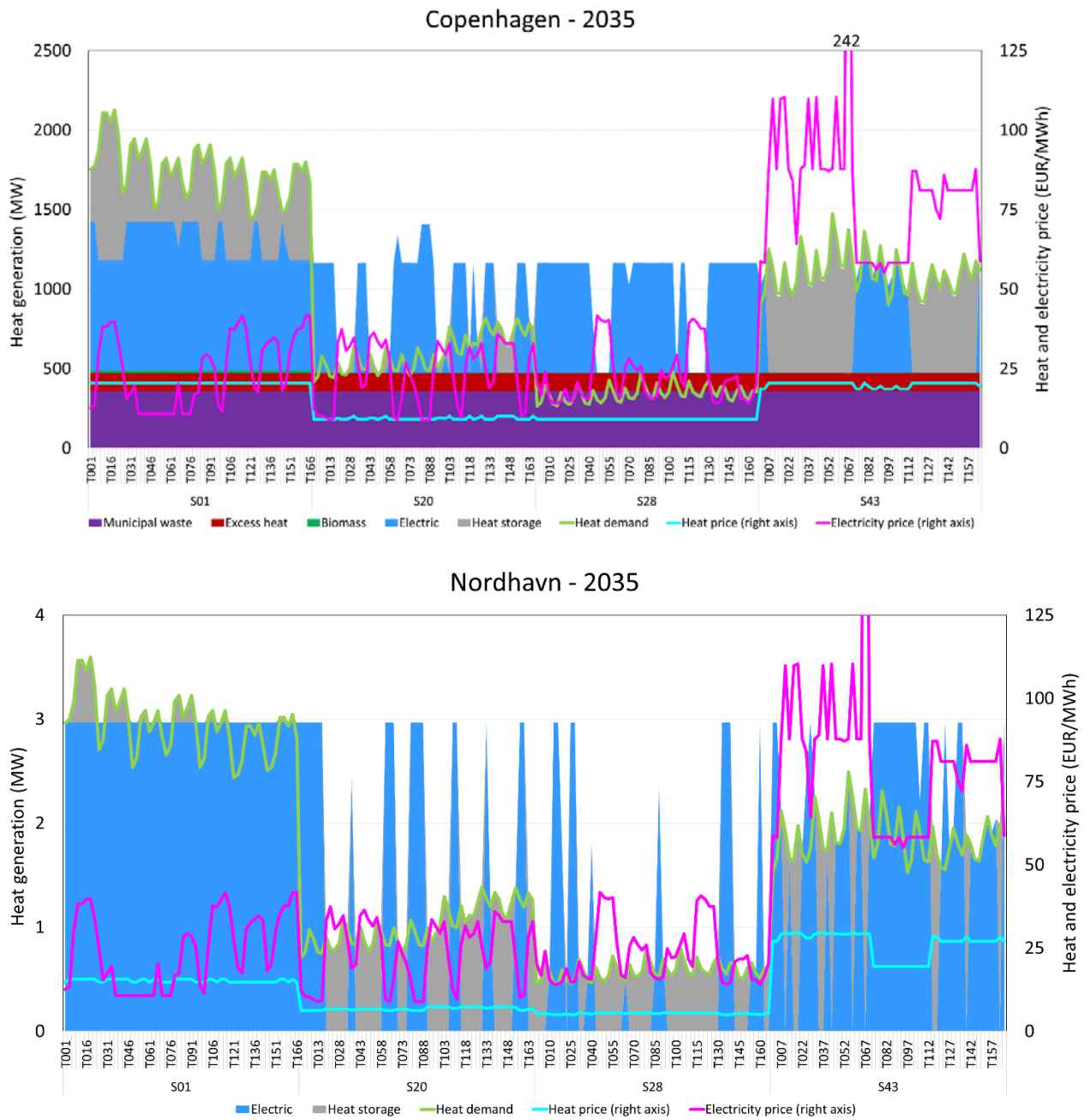
Figure 4. Dynamics between heat production and demand and electricity and heat prices for GC (top) and Nordhavn (down) in 2035 in the reference scenario.
