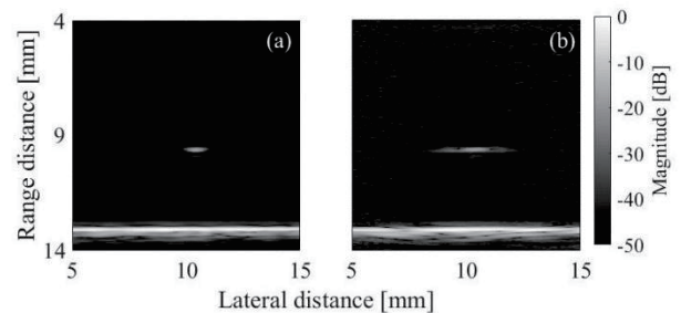
Fig. 4 B-mode images obtained with element pitch of 0.1 mm by assuming (a) a point sound source and (b) a plane sound source.
