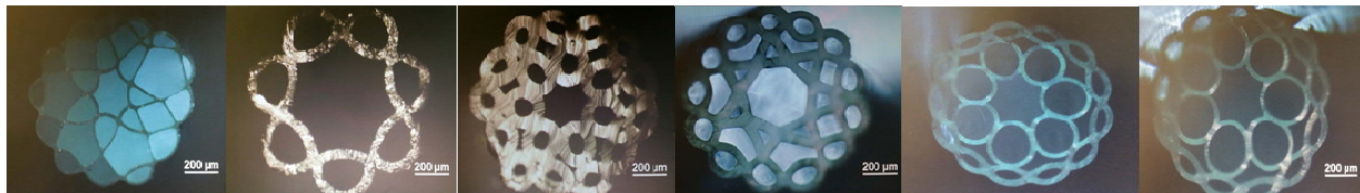
Fig. 1. Images of transverse cross-sections of a range of microstructured fibres drawn in polyurethane
