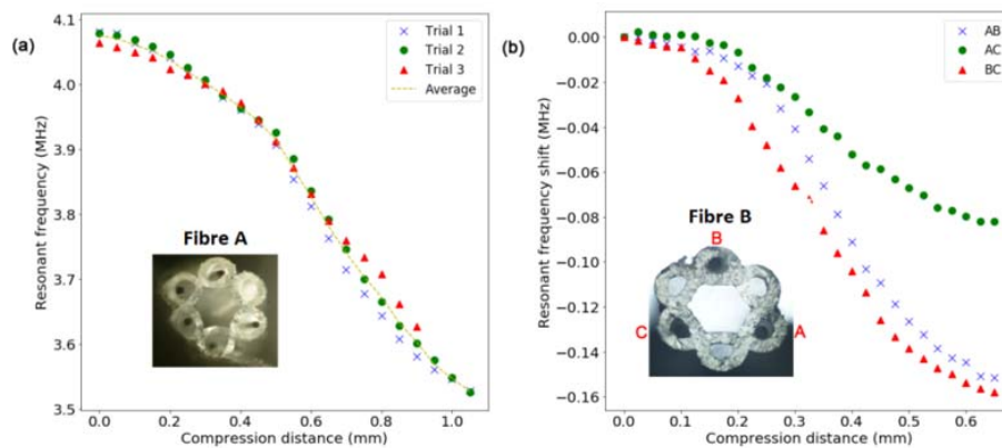
Figure 3 Response of two designs of polyurethane metal composite fibre capacitive pressure sensor [7]
