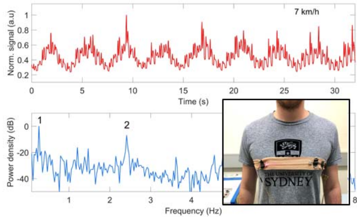
Figure 2 Time and frequency domain signals from polyurethane sensor in chest bandage (inset). Frequency plot - peak 1 is respiration, peak 2 step rate [6]
