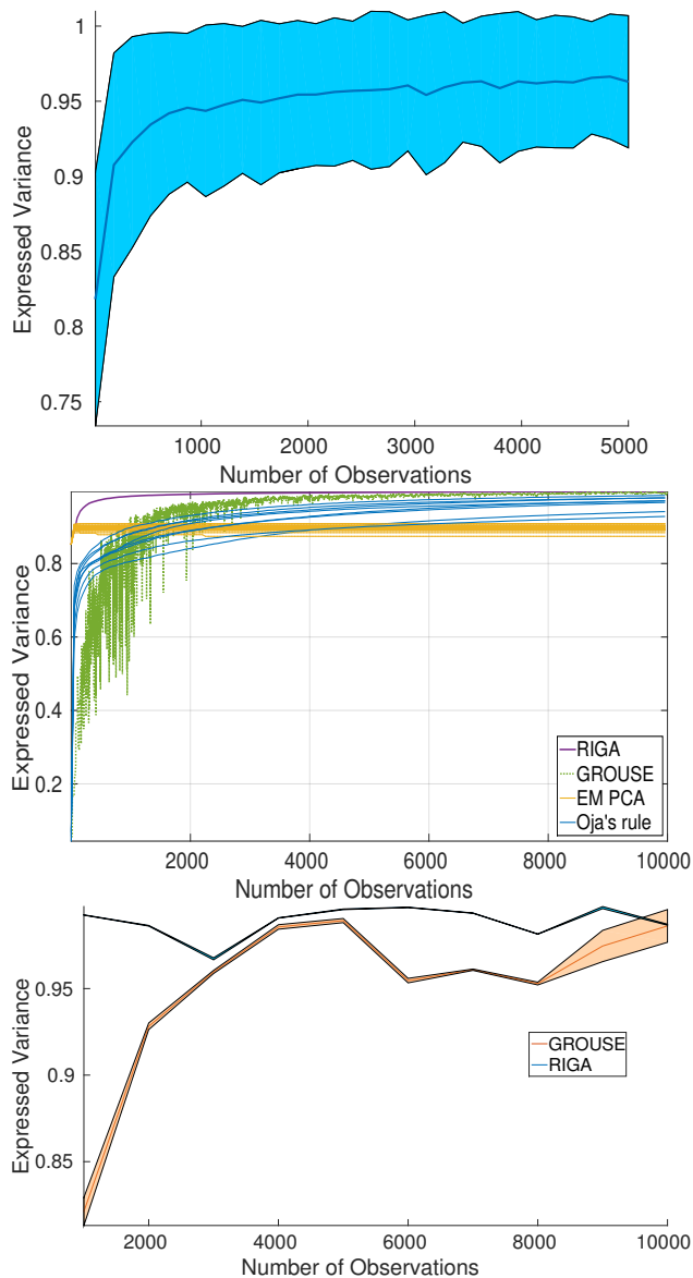
Figure 2. Expressed variance as a function of number of observations. Top : The mean and one standard deviation of the RIGA estimator computed over 150 trials. In each trial data are generated in \mathbf{R}^{50} and we estimate a K = 2 dimensional subspace. Middle : The performance of different estimators for varying step-sizes. Data are generated in \mathbf{R}^{250} and we set K = 20 . In both experiments, we observe similar trends with other values of D and K . Bottom : Stability analysis comparison of GROUSE and RIGA (for a fixed N , we randomly generate a data matrix, X , from a Gaussian distribution on \mathbf{R}^{250} . we estimate K = 20 dimensional subspace and report the mean and one standard deviation over 200 runs on X .)
