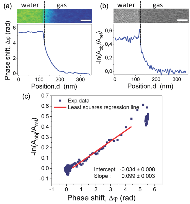
FIG. 2. Example of \lambda_{\text{IMFP}} based water MIP measurement. (a) Phase image and corresponding profile plots near a meniscus; (b) the inverse logarithm of amplitude ( A_{\text{obj}} ) normalized to region without liquid ( A_{\text{ref}} ), and corresponding profile plots. (c) Plot of correlation and linear fit to -\ln(A_{\text{obj}}/A_{\text{ref}}) vs \Delta\varphi . The scale bar is 50 nm.
