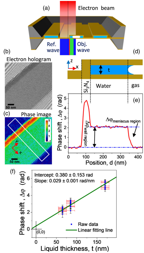
FIG. 1. Thickness based MIP measurement. (a) Illustration of the setup for nanochannel LPTEM off-axis electron holography. Interference of object and reference waves create the interference hologram in (b) of water near a nanochannel sidewall, with a stable meniscus to a bubble in the channel. (c) Reconstructed phase image with color code of \Delta\phi in radian. (d) Schematic nanochannel cross section with liquid thickness t . (e) Phase profile along the x direction from the white box in (c); \Delta\phi was averaged over 80 nm in the y direction. (f) Liquid water \Delta\phi from three channels with liquid thickness t , and linear fit \Delta\phi = C_E V_0^{\text{water}} t + a .
