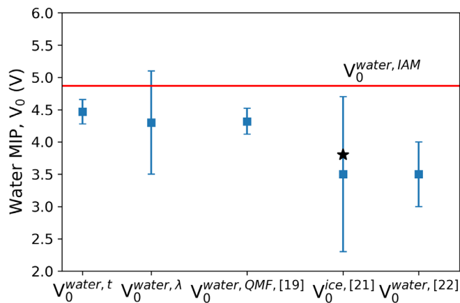
FIG. 3. Comparison of water MIP values. From the nanochannel thickness based method, V_0^{\text{water},t} ; \lambda_{\text{IMFP}} based method, V_0^{\text{water},\lambda} ; the QMF model, V_0^{\text{water},QMF} [19]; measurements on vitrified ice, V_0^{\text{ice}} [21], also scaled to liquid density ( \star ); and the water droplet estimate, V_0^{\text{water}} [22]. Red-solid line is the upper limit V_0^{\text{water},IAM} .
