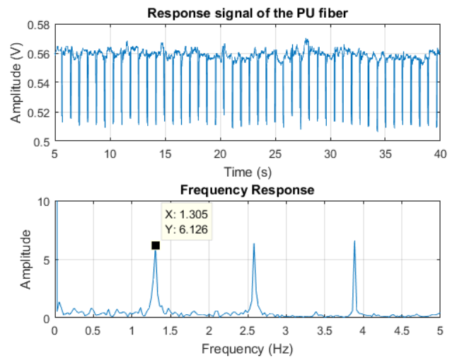
Figure 5. (a) The response of the PU fiber with the applied signal frequency to the function generator ~1.3 Hz. (b) FFT data of the time domain signal.
