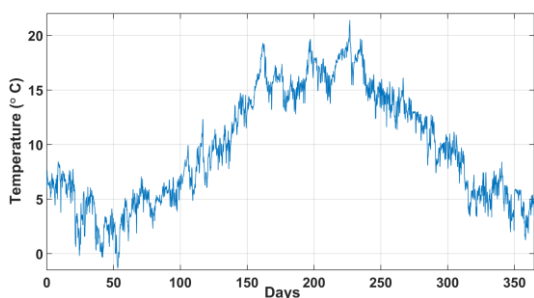
Figure 6: 2-meters above-sea temperature time series.
