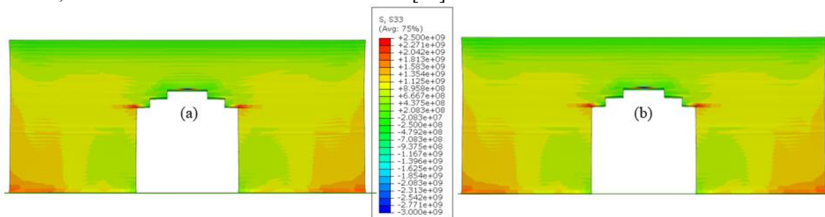
Figure 5. Stress in the bridge. (a) shows the S33 when the microstructural change is simulated, (b) the same when the microstructural change is not included.
