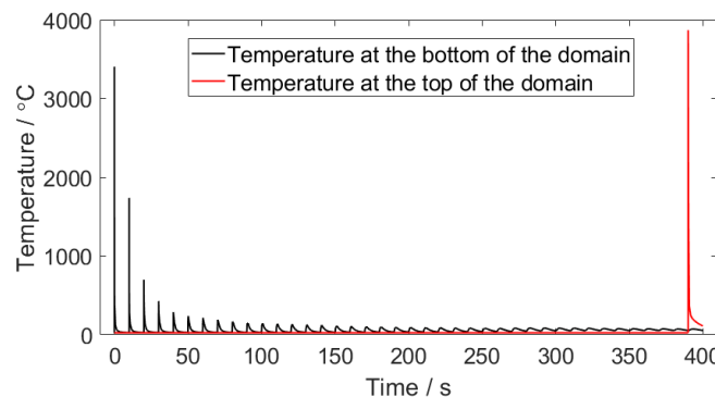
Figure 3. Temperature in the first layer of the simulation and in the final layer.
