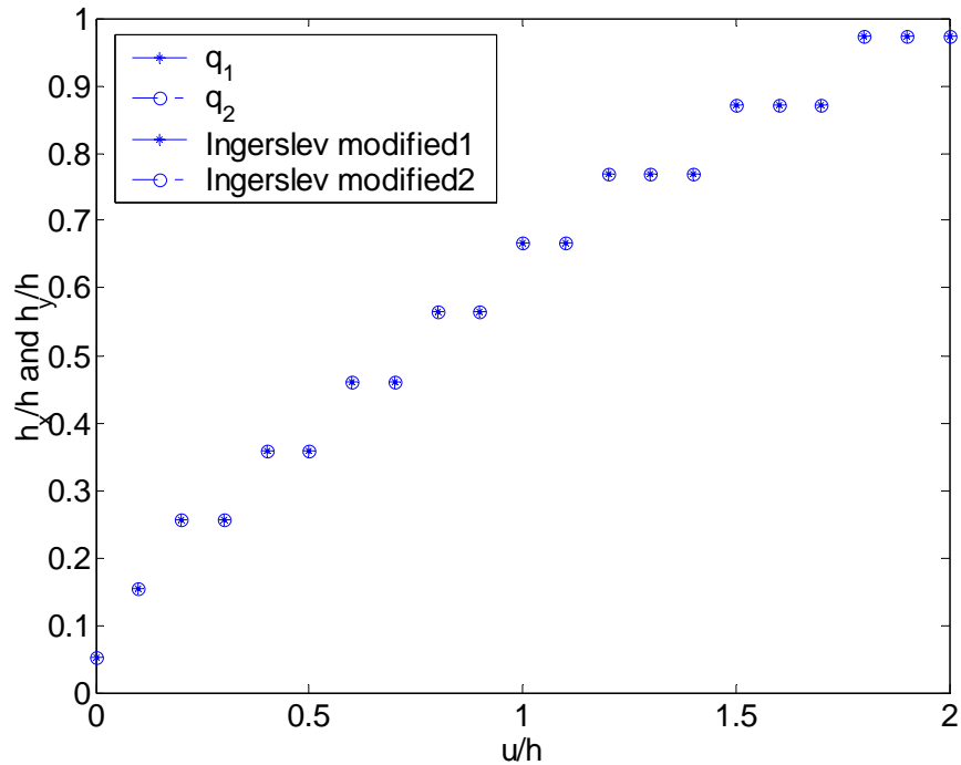
Figure 7.67 Position of the axes of rotation for failure mode 2 for a rectangular slab L_x=2000\text{mm} , L_y=2000\text{mm} , \Phi_{0x}=\Phi_{0x}'=0.15 , \Phi_{0y}=\Phi_{0y}'=0.15 , h_{cx}/h=h_{cx}'/h=h_{cy}/h=h_{cy}'/h=0 , f_c=30\text{MPa} , \sigma_x=\sigma_y=0.1f_c .
