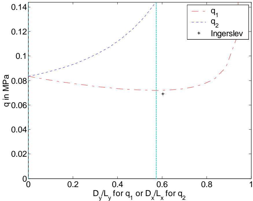
Figure 7.40. Load-carrying capacity q_1 and q_2 , according to (7.54) (dashed dotted) and (7.55) (dotted), for a square slab L_x = 2000 \text{ mm} , L_y = 16000 \text{ mm} , \Phi_{0x} = \Phi_{0x}' = 0.7 , \Phi_{0y} = \Phi_{0y}' = 0.1 , h_{cx}/h = h_{cx}'/h = h_{cy}/h = h_{cy}'/h = 0.1 , f_c = 30 \text{ MPa} and load-carrying capacity according to (7.48) or (7.50) (*).
