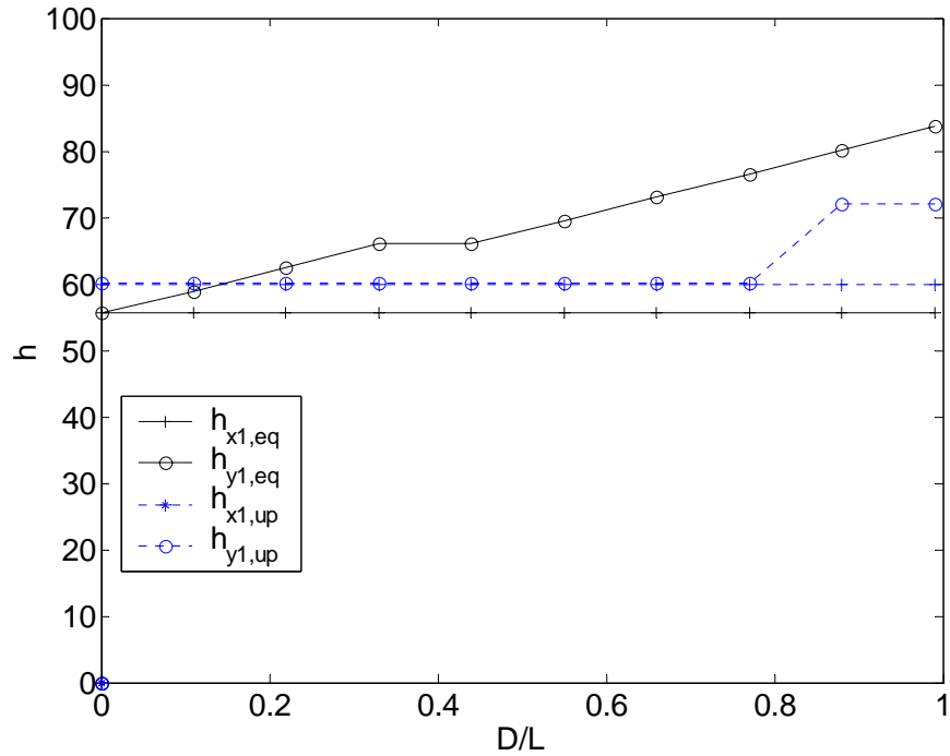
Figure 7.77. Results of calculations by equations (7.76) to (7.101) (solid) and numerical calculations (dashed) on a slab with L_x=L_y=2000\text{mm} , \Phi_{0x}=\Phi_{0x}'=\Phi_{0y}=\Phi_{0y}'=0.1 , h_c/h=0.1 , h=60\text{mm} , f_c=50\text{MPa} , u/h=1 and \sigma_x/f_c=\sigma_y/f_c=0.4 .
