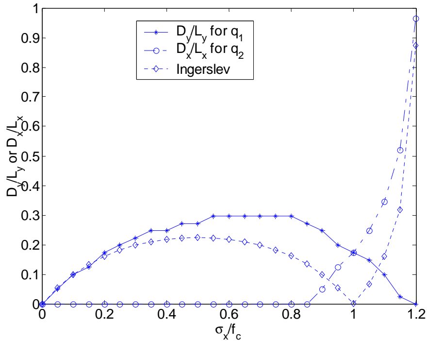
Figure 7.46. Length of the part of the yield line parallel to the axes of rotation for a rectangular slab L_x=2000\text{mm} , L_y=2000\text{mm} , \Phi_{0x}=\Phi_{0x}'=0.1 , \Phi_{0y}=\Phi_{0y}'=0.1 , h_{cx}/h=h_{cx}'/h=h_{cy}/h=h_{cy}'/h=0.1 , f_c=30\text{MPa} , h=100\text{mm} , increasing \sigma_x and \sigma_y=0 .
