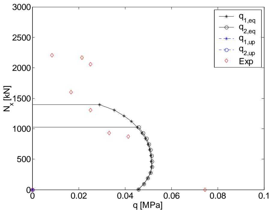
Figure 8.6. Results of calculations for a slab with f_c=60MPa , f_y=593MPa , h=60mm , h_{cm}/h=0.5 , L_x=L_y=2000mm , \Phi'_x=\Phi'_y=0.0085f_y/f_c , \Phi_x=\Phi_y=0 and \nu=0.45 .
