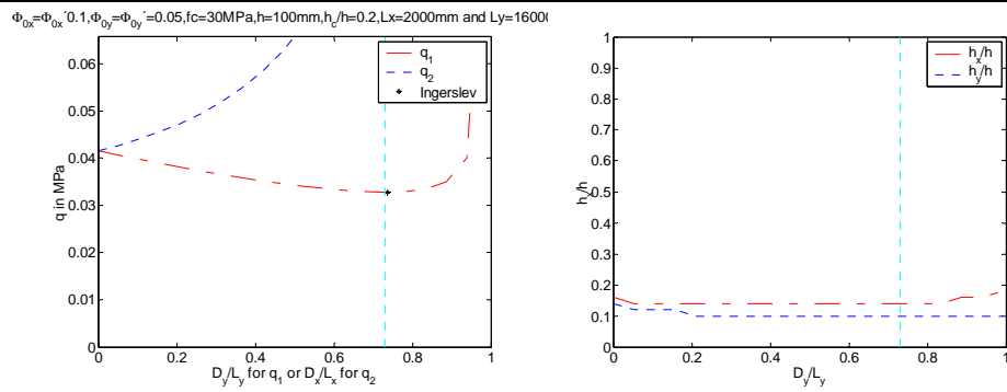
Figure 11.6. Load-carrying capacity q_1 for a rectangular slab L_x=2000\text{mm} , L_y=16000\text{mm} , \Phi_{0x}=\Phi_{0x}'=0.1 , \Phi_{0y}=\Phi_{0y}'=0.05 , h_{cx}/h=h_{cx}'/h=h_{cy}/h=h_{cy}'/h=0.2 , f_c=30\text{MPa} (solid) and load-carrying capacity according to (7.48) or (7.50) at the left hand side and position of the axes of rotation at the right hand side.
