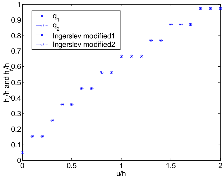
Figure 7.70 Position of the axes of rotation for failure mode 2 for a rectangular slab L_x=2000\text{mm} , L_y=2000\text{mm} , \Phi_{0x}=\Phi_{0x}'=0.15 , \Phi_{0y}=\Phi_{0y}'=0.25 , h_{cx}/h=h_{cx}'/h=h_{cy}/h=h_{cy}'/h=0 , f_c=30\text{MPa} , \sigma_x=0.1f_c , \sigma_y=0 .
