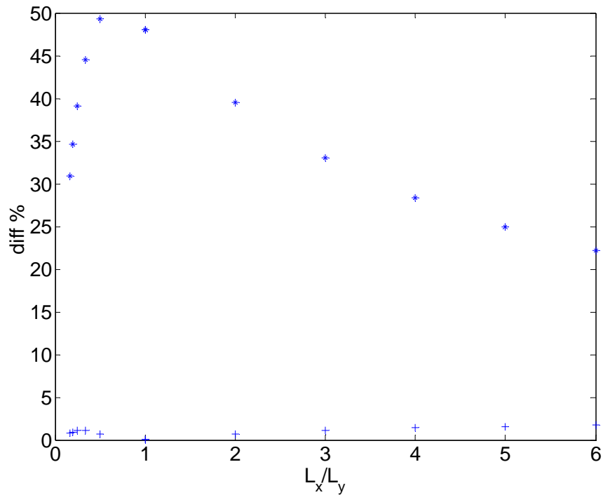
Figure 7.51. Maximum (*) and minimum (+) difference between the two calculation methods for a rectangular slab L_x=2000\text{mm} , \Phi_{0x}=\Phi'_{0x}=0.05 , \Phi_{0y}=\Phi'_{0y}=0.05 , h_{cx}/h=h'_{cx}/h=h_{cy}/h=h'_{cy}/h=0.1 , f_c=30\text{MPa} , h=100\text{mm} , \sigma_x variation from 0 to f_c(1+\Phi_{0x}+\Phi'_{0x}) , \sigma_y=0 and different L_x/L_y ratios.
