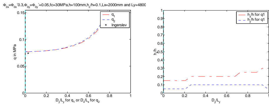
Figure 11.8. Load-carrying capacity q_1 for a rectangular slab L_x=2000\text{mm} , L_y=4800\text{mm} , \Phi_{0x}=\Phi_{0x}'=0.3 , \Phi_{0y}=\Phi_{0y}'=0.05 , h_{cx}/h=h_{cx}'/h=h_{cy}/h=h_{cy}'/h=0.1 , f_c=30\text{MPa} (solid) and load-carrying capacity according to (7.48) or (7.50) at the left hand side and position of the axes of rotation at the right hand side.
