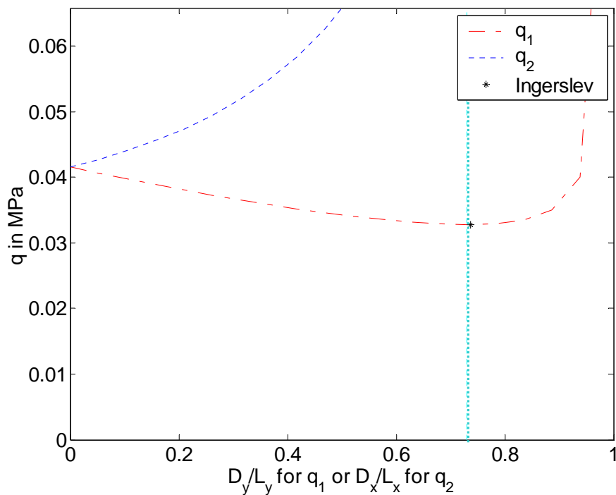
Figure 7.37. Load-carrying capacity q_1 and q_2 , according to (7.54) (dashed dotted) and (7.55) (dotted), for a square slab L_x=2000\text{mm} , L_y=16000\text{mm} , \Phi_{0x}=\Phi_{0x}'=0.1 , \Phi_{0y}=\Phi_{0y}'=0.05 , h_{cx}/h=h_{cy}/h=0.2 , f_c=30\text{MPa} and load-carrying capacity according to (7.48) or (7.50) (*).
