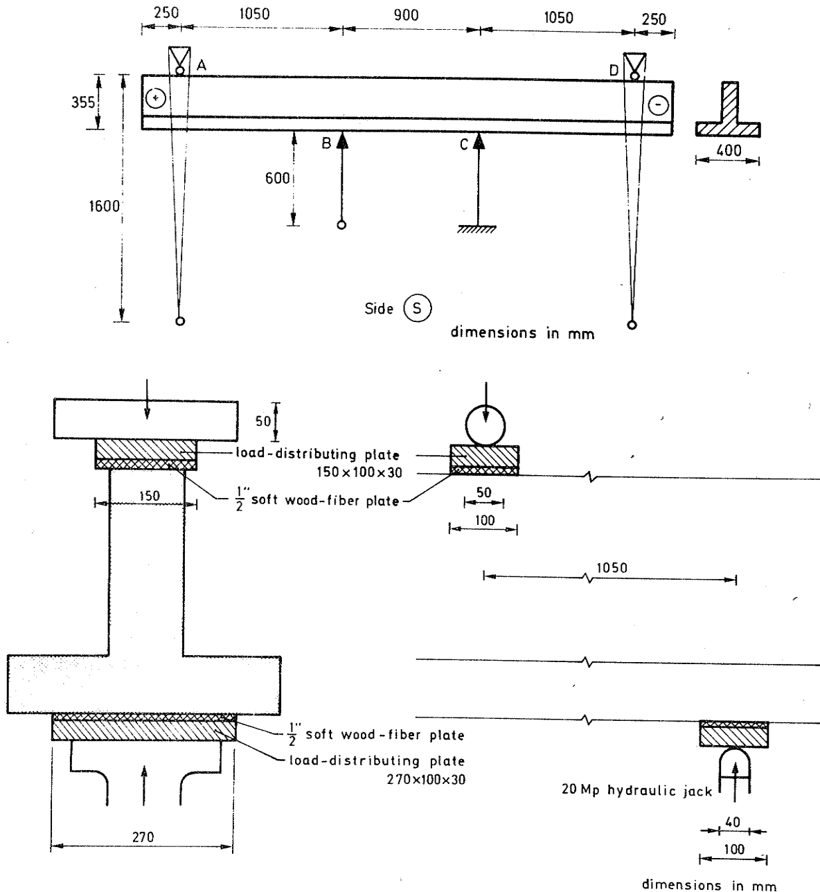
Fig.2.7: Loading arrangement
