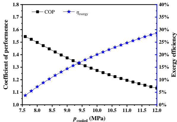
Fig 7 Variation of the coefficient of performance and the exergy efficiency with the cooled pressure
