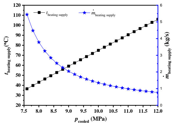
Fig 6 Variation of the temperature and mass flow rate of the supplied hot water with the cooled pressure
