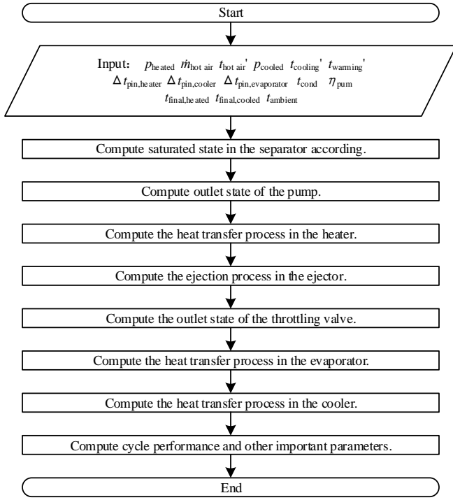
Fig 3 Flow chart of the calculation process
