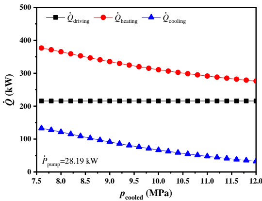
Fig 5 Variation of the heat capacities with the cooled pressure
