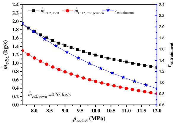
Fig 4 Mass flow rate of CO 2 and ejection entrainment with the cooled pressure
