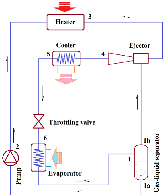
Fig 1 Flow chart of the heat-driven CO 2 high temperature heat pump
