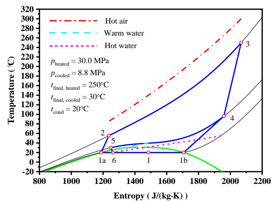
Fig 2 Thermodynamic process of the heat-driven CO 2 high temperature heat pump
