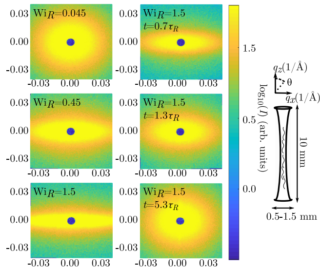
FIG. 2. Two-dimensional SANS data on uniaxially extended polystyrene and experimental geometry. Intensities are plotted on a logarithmic scale and the units of q_x and q_z are 1 \text{ \AA}^{-1} . The left column shows increasing Wi_R and the right column increasing t following extension at Wi_R = 1.5 . The fully relaxed pattern for Wi_R = 1.5 and t = 21.3\tau_R is omitted. The stretching direction and polar angle \theta are defined on the filament cartoon.
