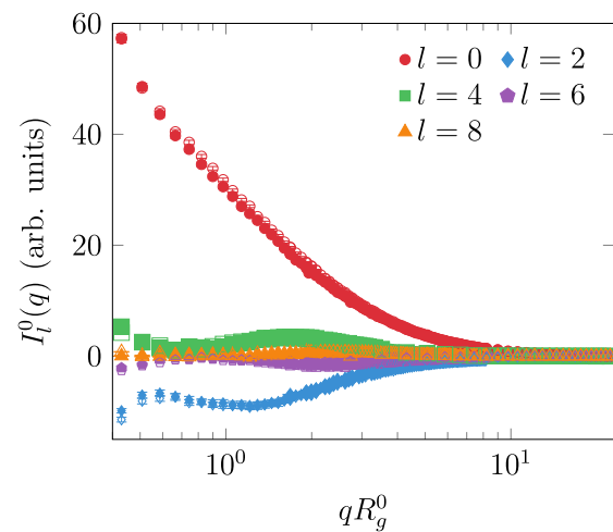
FIG. 4. Comparison of the overlapping fingerprints for molecular conformations with a cylinder length slightly larger than L_0 , Wi_R = 0.15 and t = 0.7\tau_R ( Wi_R = 0.45 and Wi = 3 ), in closed (open) symbols.
