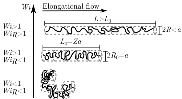
FIG. 1. Steady-state molecular conformation for elongation at increasing Weissenberg numbers Wi = \dot{\epsilon}\tau_d and Wi_R = \dot{\epsilon}\tau_R , where \dot{\epsilon} is the deformation rate and \tau_d and \tau_R are the reptation and Rouse times, respectively. The Z tube segments are marked by dashed lines.
