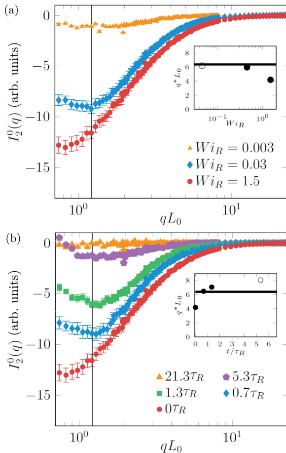
FIG. 3. Expansion coefficient I_2^0(q) as a function of scattering vector made dimensionless with the length of the fully oriented tube qL_0 for (a) varying Rouse-Weissenberg number Wi_R and (b) varying duration of stress relaxation t following a deformation with Wi_R = 1.5 . Vertical lines show the location of the minimum for the fully oriented chain from the cylinder model. The insets show q^* that minimizes I_2^0(q) (a) as a function of Wi_R and (b) as a function of t relative to the Rouse time \tau_R . Open symbols indicate an uncertain value due to shallowness or crack scattering. The fully drawn horizontal lines show the minimum position for the fully oriented chain. All samples are stretched to a final Hencky strain of \varepsilon = 3 .
