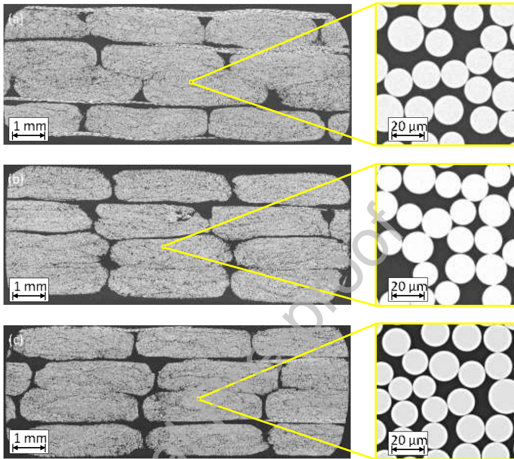
Figure 2: Scanning electron microscope images of Sample-A (a), Sample-G (b) and Sample-E (c) scanned at DTU Roskilde, Denmark with a VEGA3 SBU. With a pixel size of 250-350 nm the fibre diameter will cover 50-70 pixels
