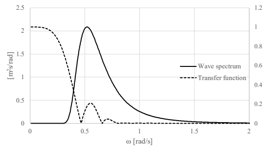
Fig. 1 Transfer function of heave motion and wave spectrum
