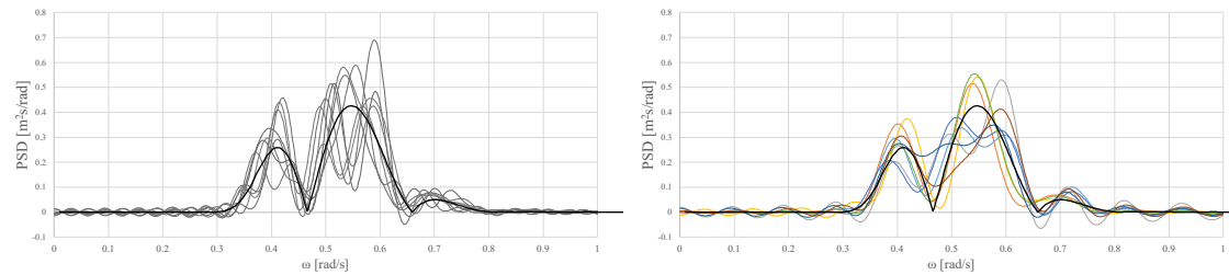
a) Fourier transform of sample ACF
