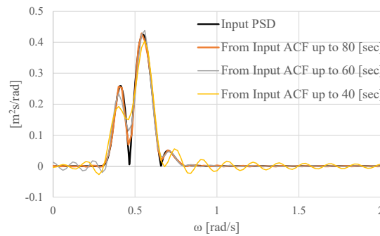
Fig. 2 Power spectral density of heave motion based on transfer function and wave spectrum
