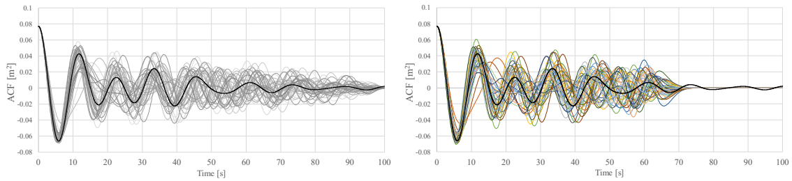
a) Sample ACF
