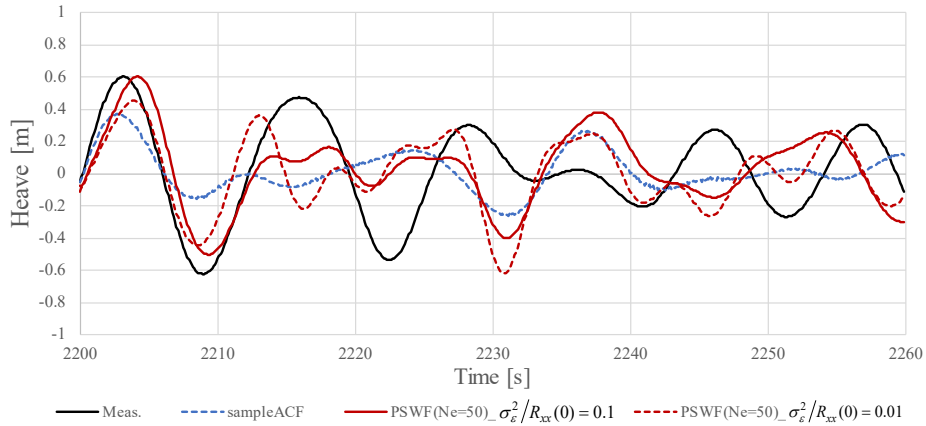
Fig. 21 Comparisons of ACF based prediction results starting from 2200 [s] between sample ACF and PSWF-based ACF with Gaussian noise. Sample ACF and PSWF-based ACF are calculated from recent 200 [s] measurements (from 2000-2200[s])
