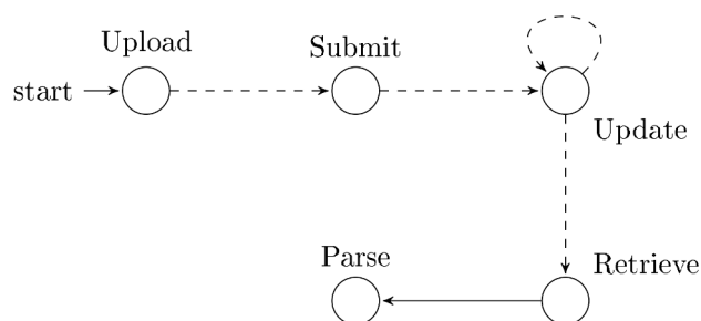
Fig. 3. Substates of the calculation job. A remote job is executed by transitioning through these states with each dashed transition occurring only when an open transport is available (prior to which the process is in a waiting state which is not shown).
