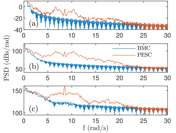
Fig. 4. Benchmark controller (BMC) vs Perturbation-based ESC (PESC). PSD of pitch reference 1 (a), thrust force 1 (b) and tower root moment (c).
