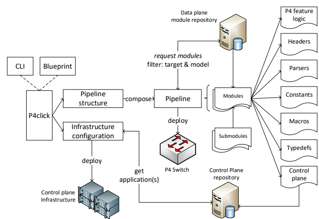
Figure 2: Integration of the modularity engine (P4click) with the control and data plane infrastructure.
