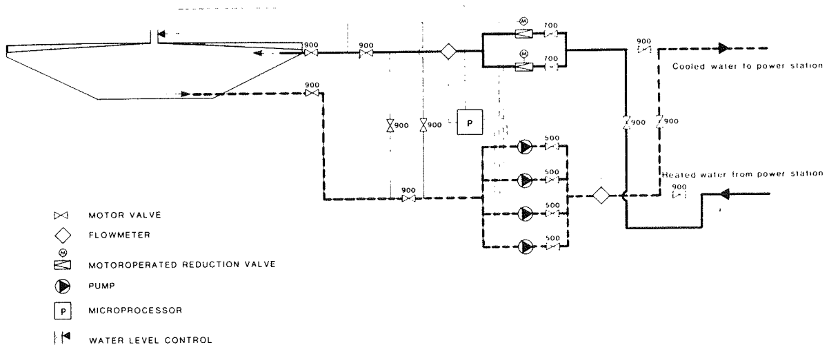
Figure 3. Pumpstation. Principal diagram. Charge operation.
