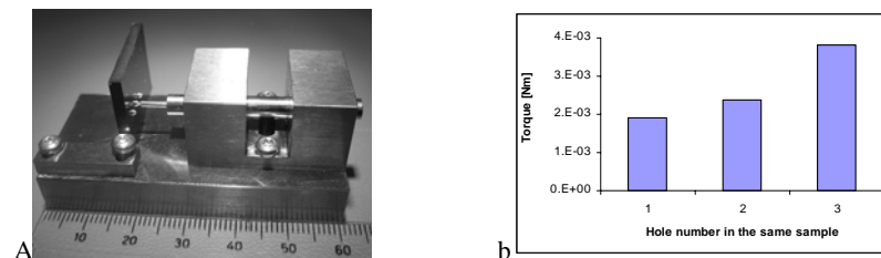
Figure 2: a - the picture of the torque measurement device, b –the results for torque measurements in POM
