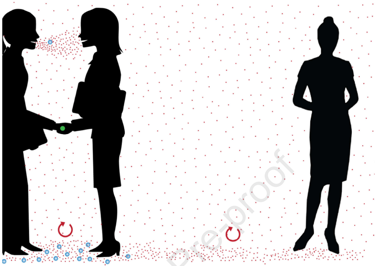
Figure 1. Showing the range of respiratory particles and potential spread over distance. Blue particles: 'droplets' typically >100 \mu\text{m} diameter that fall to the floor under gravity within 2 m of the source. Red particles: 'aerosols' typically <100 \mu\text{m} that stay suspended for longer, but eventually fall to the ground if the air is motionless for long enough (at least 30 minutes).
